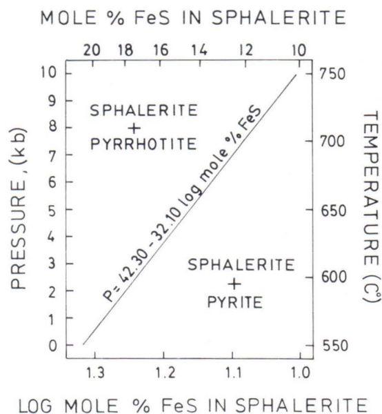
Fig. 3. Pressure-log mole per cent FeS projection onto the FeS-ZnS join of the temperature-independent portions of the sphalerite + pyrite + hexagonal pyrrhotite solvus isobars. Temperature scale gives the upper limit of the temperature-independent portion. After Hutchison and Scott (1981).
