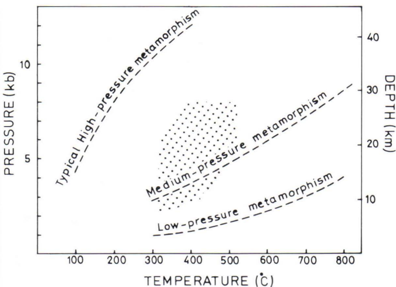
Fig. 6. pT diagram showing the main types of metamorphism after Miyashiro (1973). The shaded area represents the suggested model pressure-temperature conditions of metamorphism in the sulphide ores.
