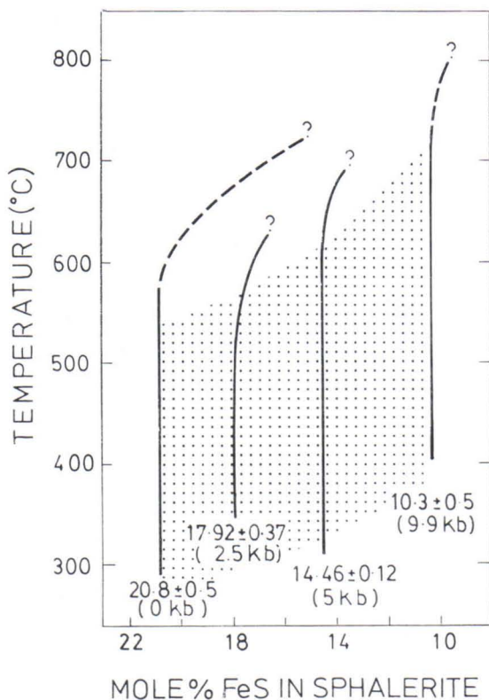
Fig. 2. T-X projection onto the FeS-ZnS join of the sphalerite + hexagonal pyrrhotite + pyrite solvus isobars. Temperature-independent portion is indicated by the shaded area. Modified after Lusk and Ford (1978).
