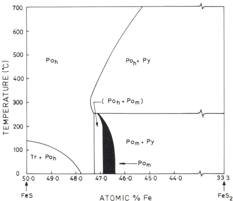
Fig. 4. Simplified relations in the central portion of the Fe-S system. Hexagonal pyrrhotite ( \text{Po}_h ), monoclinic pyrrhotite ( \text{Po}_m ), pyrite (Py), troilite (Tr). Modified after Scott et al. (1977).
