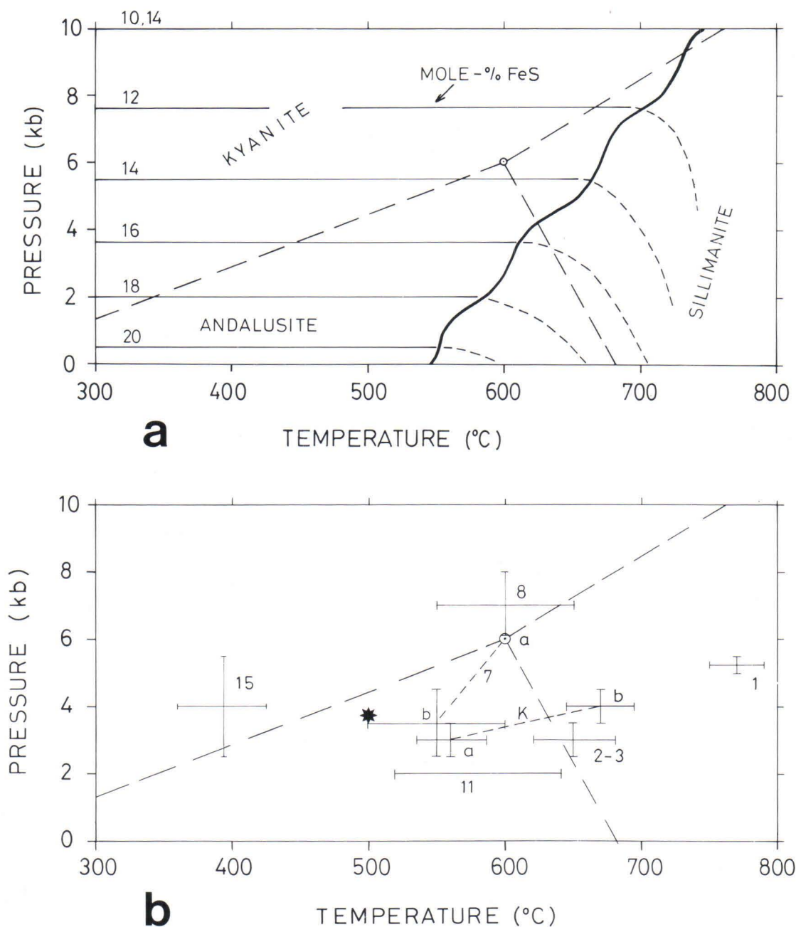
Fig. 5. a) pT projection of sphalerite isobars from Fig. 2 superimposed on the Al_2SiO_5 diagram of Winkler (1974). Wavy line marks the upper limit of the temperature-independent portion of the sphalerite geobarometer.
